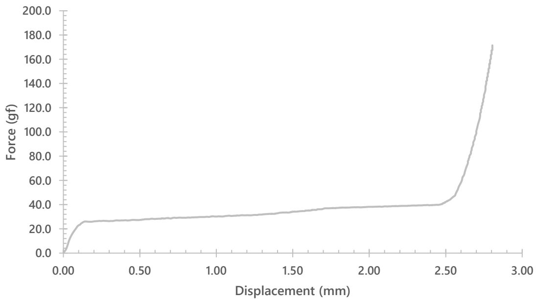
Kailh Low Profile Islet (Upstroke)
